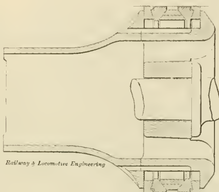
FIG. 15. "AMERICAN" TWO RING COMPLETE.
